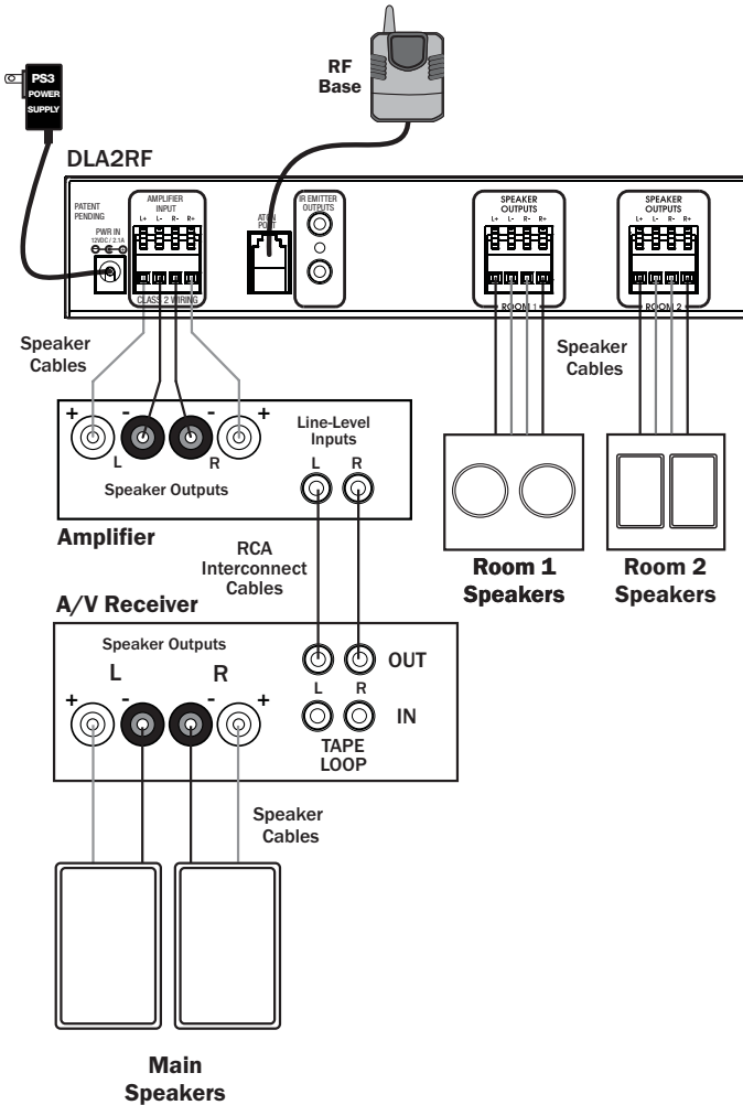
Figure 2-3: External Amplifier - A/V Receiver Tape Loop Application
